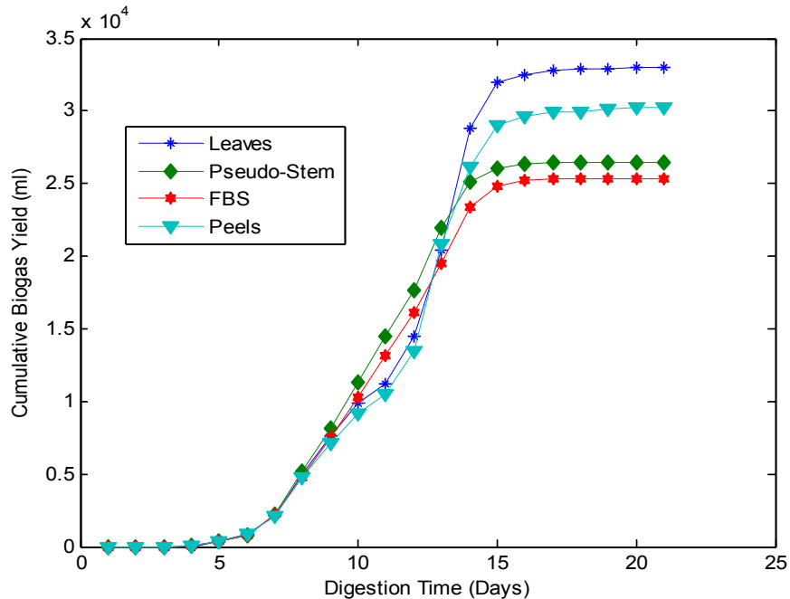
Fig. 3. Cumulative biogas production for the different banana plant substrates for 21 days
