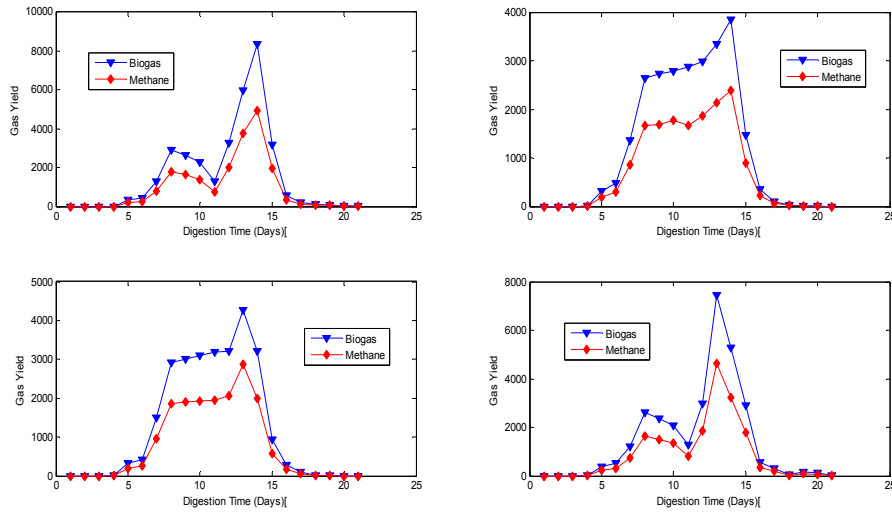
Fig. 6. Comparison between biogas and methane production
