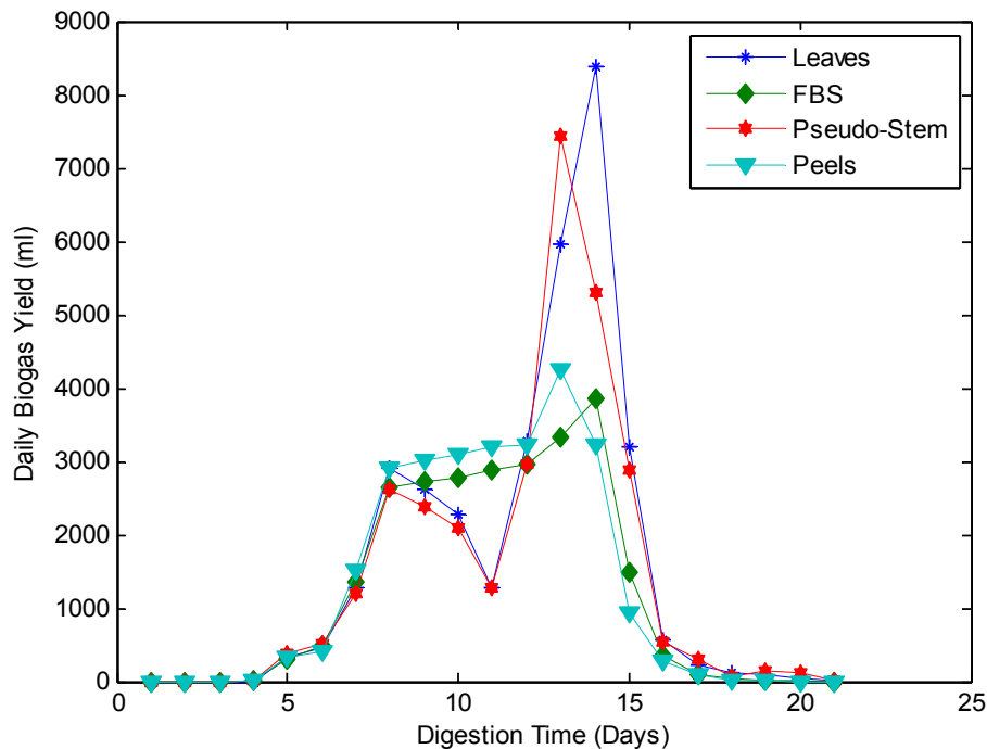
Fig. 2. Daily biogas yield against digestion days for the different banana substrates
