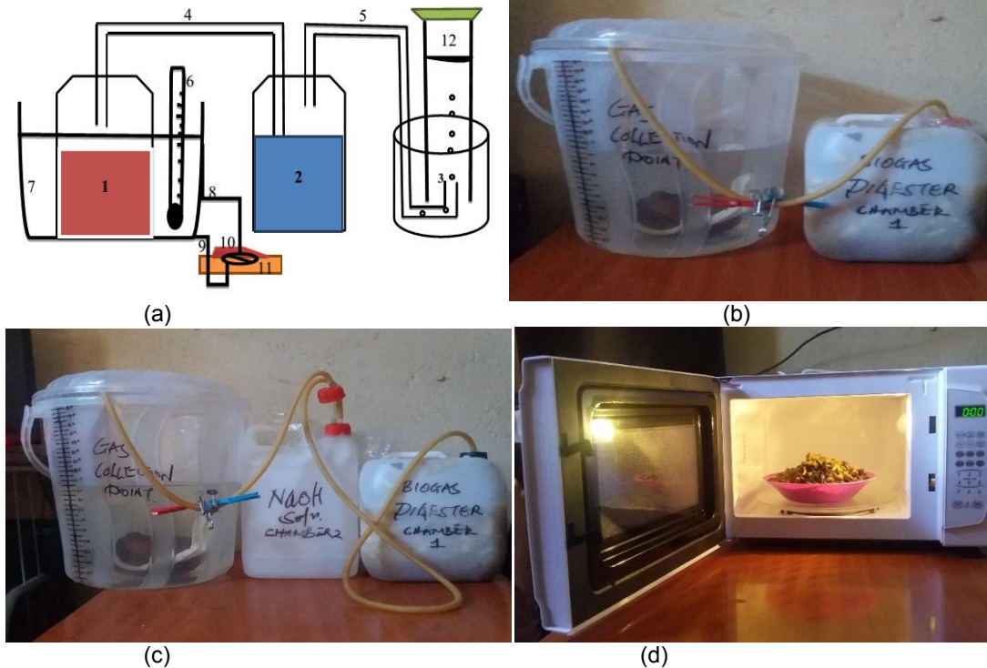
Fig. 1. Experimental set up of the digester: a schematic diagram (a), photo of the real set up of biogas collection (b), photo of methane collection (c), and photo for moisture content and total solid determination. In (a): 1 is the digester, 2 is the sodium hydroxide, 3 is the Water, 4 is Biogas, 5 is methane, 6 is the thermometer, 7 is Water, 8 is hot water, 9 is cold water, 10 is the Iron box 11 is the coil, 12 is methane
